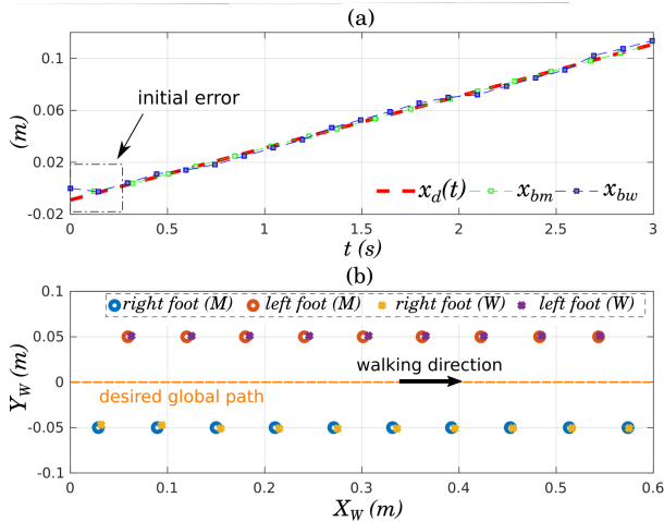
Fig. 2. Global-position tracking results in MATLAB and Webots simulations. The initial global-position tracking error is set as x_{bm}(0) - x_d(0) = x_{bw}(0) - x_d(0) = -1 cm, which is approximately \frac{1}{3} of the step length. (a) Tracking results of x_d(t) , x_{bm}(t) and x_{bw}(t) are the actual global-position trajectories along \Gamma_d obtained in MATLAB and Webots simulations, respectively. Both of them demonstrate satisfactory tracking of the desired trajectory x_d(t) . (b) Tracking results of \Gamma_d . left foot (M) and right foot (M) are the actual support-foot placements in MATLAB simulations, and left foot (W) and right foot (W) are those in Webots simulations. Both of them indicate satisfactory tracking of the desired path \Gamma_d , which is the X_W -axis of the world coordinate frame.
